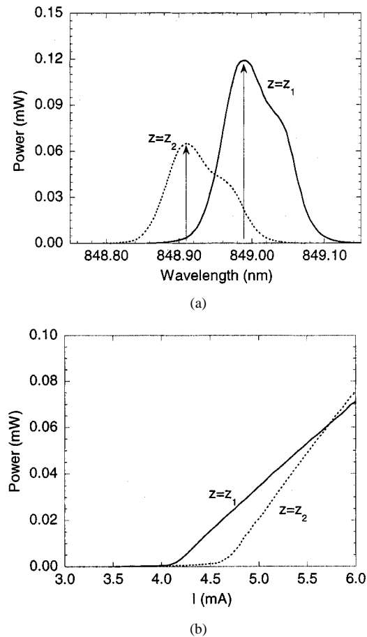
Fig. 3. (a) Measured spectra at arbitrary fiber facet positions z = z_1 and z = z_2 at I = 5.0 mA. (b) Measured L – I curves at z = z_1 and z = z_2 . At z = z_1 , I_{th} = 4.1 mA and C_{LI}\eta_d = 0.027 and for z = z_2 , I_{th} increases to 4.5 mA and C_{LI}\eta_d increases to 0.036.
