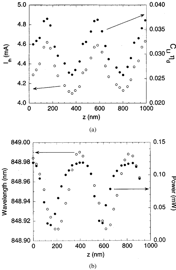
Fig. 4. (a) Measured threshold current and C_{LI}\eta_d as a function fiber facet position z . (b) Measured resonant wavelength and peak fundamental mode power as a function of fiber facet position z .
