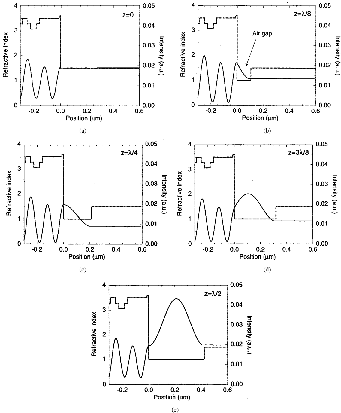
Fig. 2. Refractive index of VCSEL and fiber and intensity standing-wave patterns for: (a) z = 0 ; (b) z = \lambda/8 ; (c) z = \lambda/4 ; (d) z = 3\lambda/8 ; and (e) z = \lambda/2 . The output intensity in the fiber varies periodically as a function of z .
