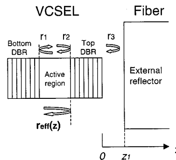
Fig. 1. Schematic of the VCSEL feedback model which consists of bottom and top DBRs with facet field reflectivities r_1 and r_2 and an external fiber reflector with reflectivity r_3 . An effective reflectivity r_{\text{eff}}(z) is defined to take into account both r_2 and r_3 . A linear change in position of the external reflector z results in a periodic change in magnitude and phase of the r_{\text{eff}}(z) .
