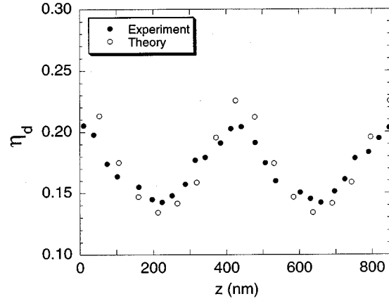
Fig. 7. Experimental and theoretical differential quantum efficiency \eta_d as a function of fiber facet position z .
