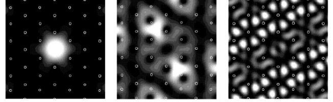
Fig. 5. Optical field distributions of the three lowest order modes are calculated for the structure with b/a of 0.1. This structure with V_{\text{eq}} of 2.2 has only one confined mode, which is doubly degenerated.
