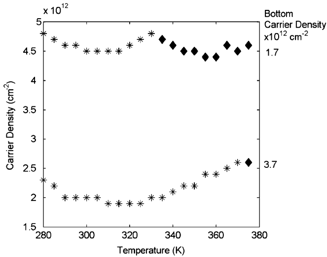
Fig. 5. Modeled threshold carrier density of the top cavity and dominant longitudinal mode for various biases on the bottom cavity. An asterisk indicates that the short wavelength lased, and a diamond indicates that the long wavelength lased. Threshold gain is assumed to be at 1500 \text{ cm}^{-1} .
