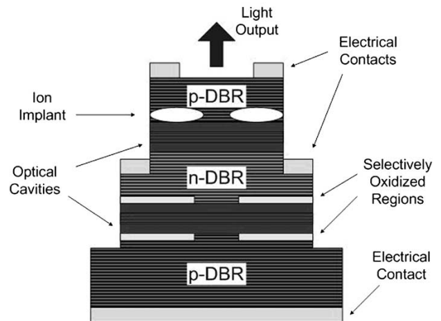
Fig. 1. Structure of CRVCL [7].
