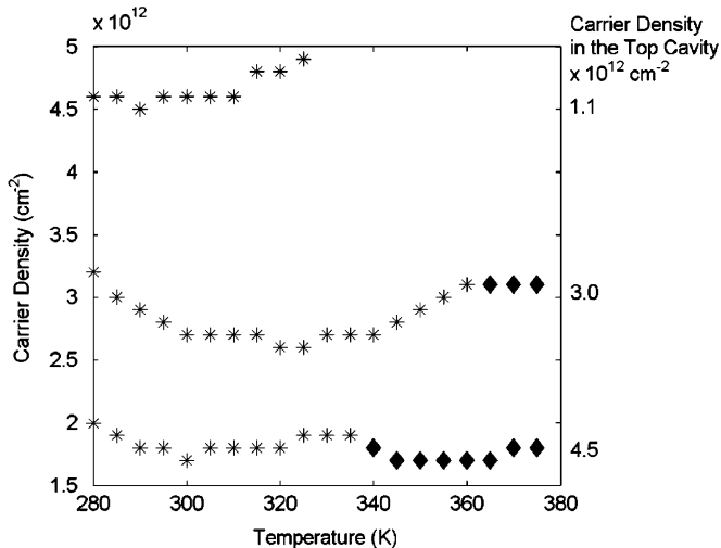
Fig. 8. Modeled threshold carrier density of the top cavity and dominant longitudinal mode for various biases on the bottom cavity. An asterisk indicates that the short wavelength lased, and a diamond indicates that the long wavelength lased. Threshold gain is assumed to be at 1500 \text{ cm}^{-1} .
