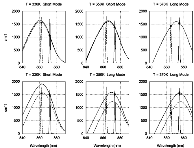
Fig. 7. Plots of effective gain and cavity resonances. The intersection of each cavity resonance with its effective gain curve is marked with a point. The top plots correspond 3.0 \times 10^{12} carriers/ \text{cm}^2 in the top cavity, and the bottom plots correspond to 4.5 \times 10^{12} carriers/ \text{cm}^2 in the top cavity. The bottom cavity gain is increased until threshold ( 1500 \text{ cm}^{-1} ) is met as plotted here. Each column corresponds to a different temperature as labeled.
