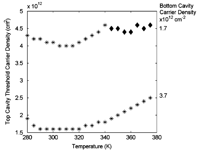
Fig. 6. Modeled threshold carrier density of the top cavity and dominant longitudinal mode for various biases on the bottom cavity. An asterisk indicates that the short wavelength lased, and a diamond indicates that the long wavelength lased. Threshold gain is assumed to be at 1300 \text{ cm}^{-1} for the short mode and 1500 \text{ cm}^{-1} for the long mode.
