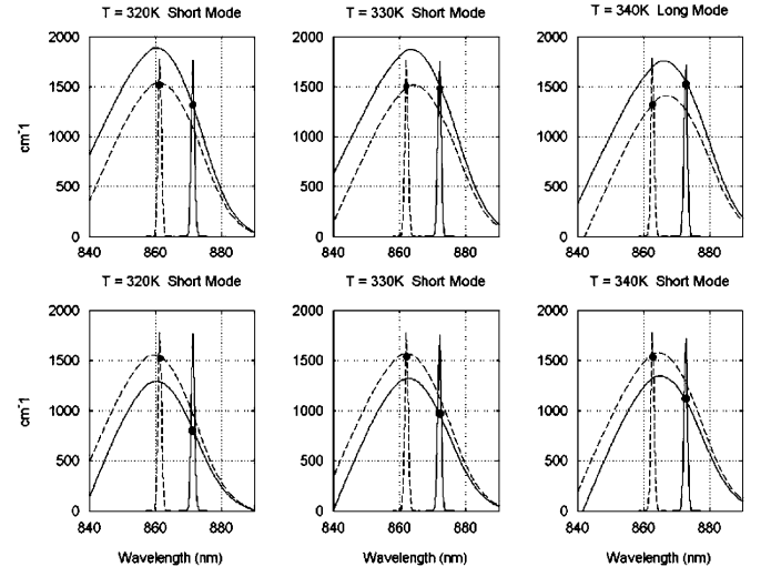
Fig. 4. Plots of effective gain and cavity resonances. The intersection of each cavity resonance with its effective gain curve is marked with a point. The top plots correspond 1.7 \times 10^{12} carriers/cm -2 in the bottom cavity, and the bottom plots correspond to 3.7 \times 10^{12} carriers/cm -2 in the bottom cavity. The top cavity gain is increased until threshold ( 1500 \text{ cm}^{-1} ) is met as plotted here. Each column corresponds to a different temperature as labeled.
