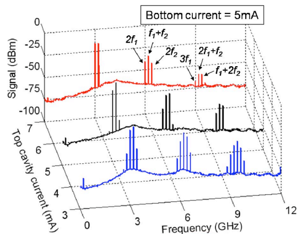
Fig. 4. RF spectra of the CRVCL light output as a function of the top cavity current with bottom cavity current held constant.
