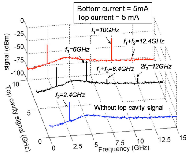
Fig. 5. RF spectra of the CRVCL light output as a function of the frequency of the microwave signal injected into the top cavity, given a fixed microwave signal in the bottom cavity.
