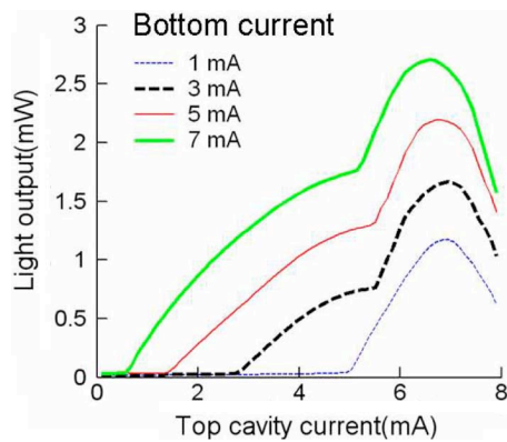
Fig. 2. Light output versus top cavity current with different dc current in the bottom cavity.
