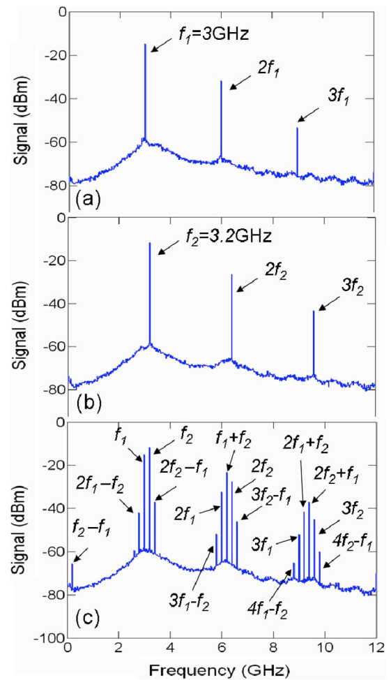
Fig. 3. RF spectrum of the CRVCL light output when only the (a) top or (b) bottom cavity is directly modulated, and (c) both cavities are modulated simultaneously.
