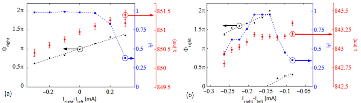
FIG. 4. Phase, coherence, and wavelength vs. current injection difference for the (a) out-of-phase and (b) in-phase VCSEL array.
