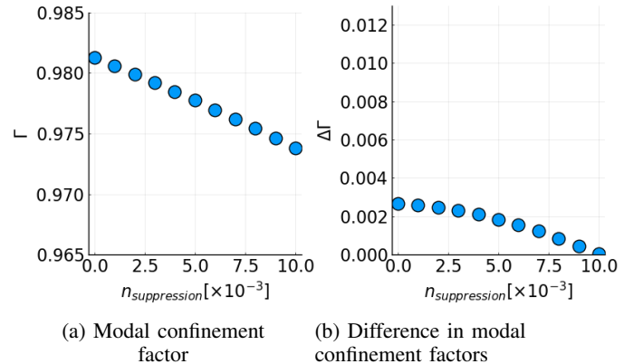
Fig. 9: The maximal modal confinement and the confinement factor difference as a function of cavity index suppression.
